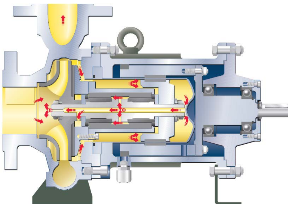
Figure 9 – Typical Magnetic Drive Pump
