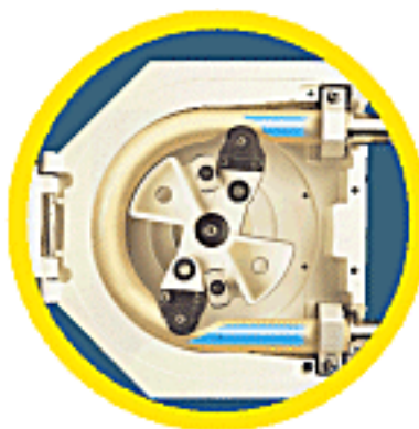
Figure 27 – Typical Two-Roller Peristaltic Pump
