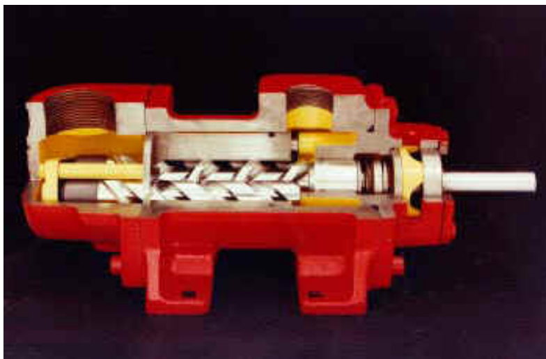
Figure 25 – Typical Screw Pump
