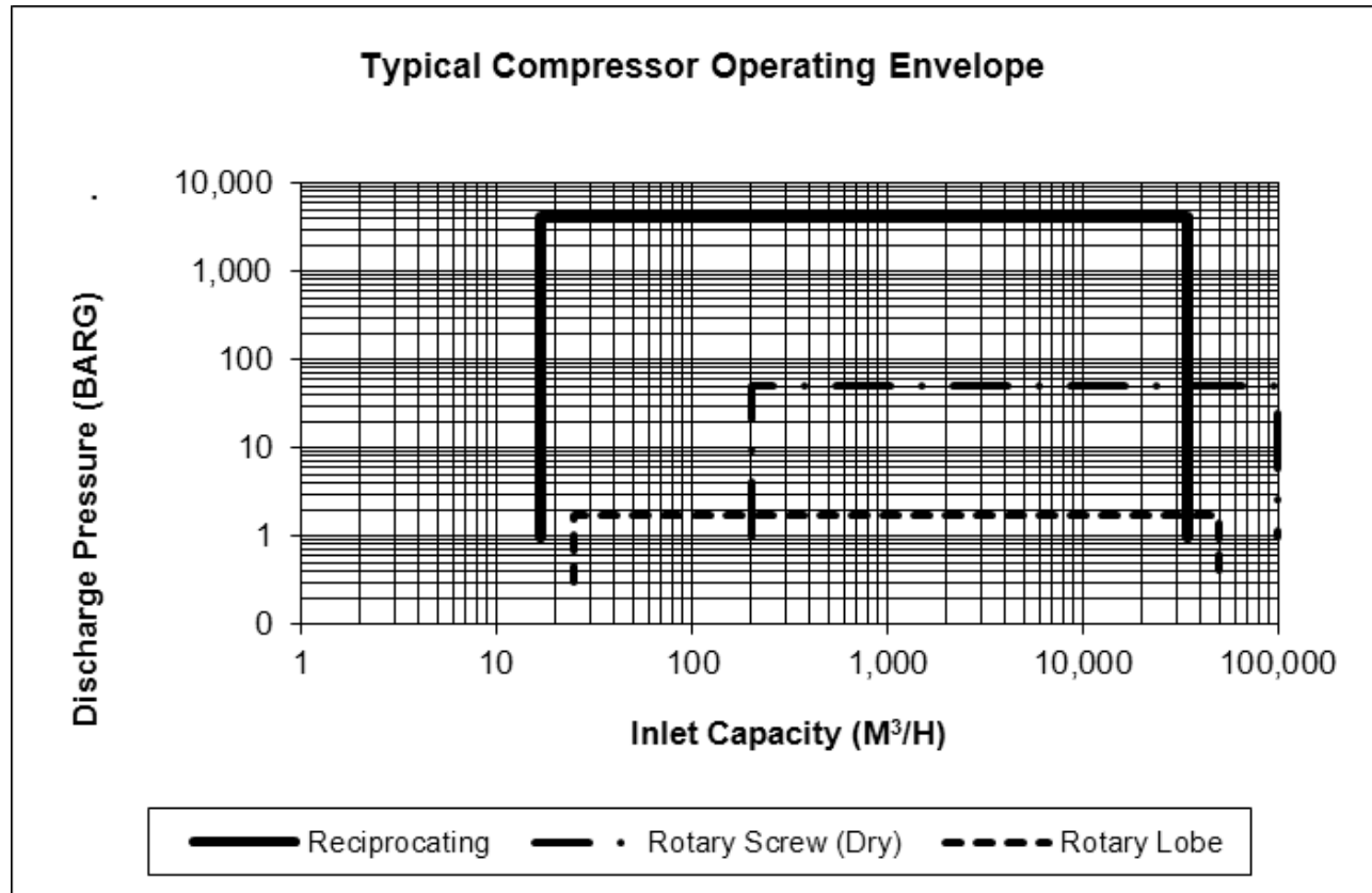
Typical Operating Envelope of Reciprocating, Rotary Screw (Dry), and Rotary Lobe (Metric)
