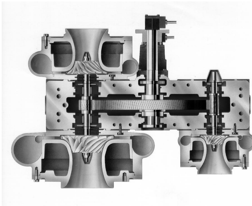
Figure 4. Typical Integrally Geared Centrifugal Compressor
